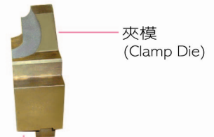
夾模 (拉彎) (Clamp Die/Draw Bending)
