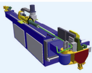
彎管虛擬 3D Simulation
