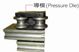
導模 (拉彎) (Pressure Die/Draw Bending)
