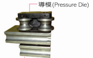
導模 (拉彎) (Pressure Die/Draw Bending)
